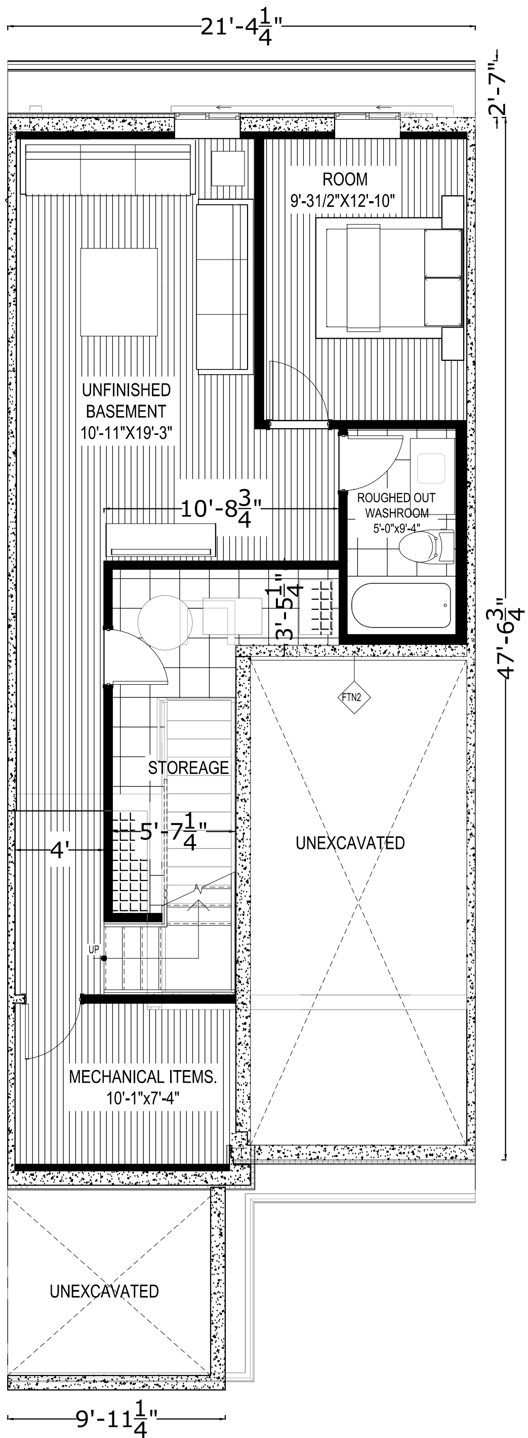
MODEL A -BASEMENT FLOOR PLAN
